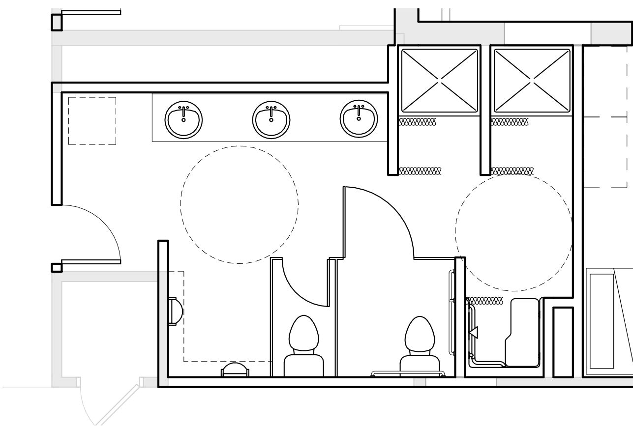
③ RESTROOM OPTION 2 1/4" = 1'-0"
