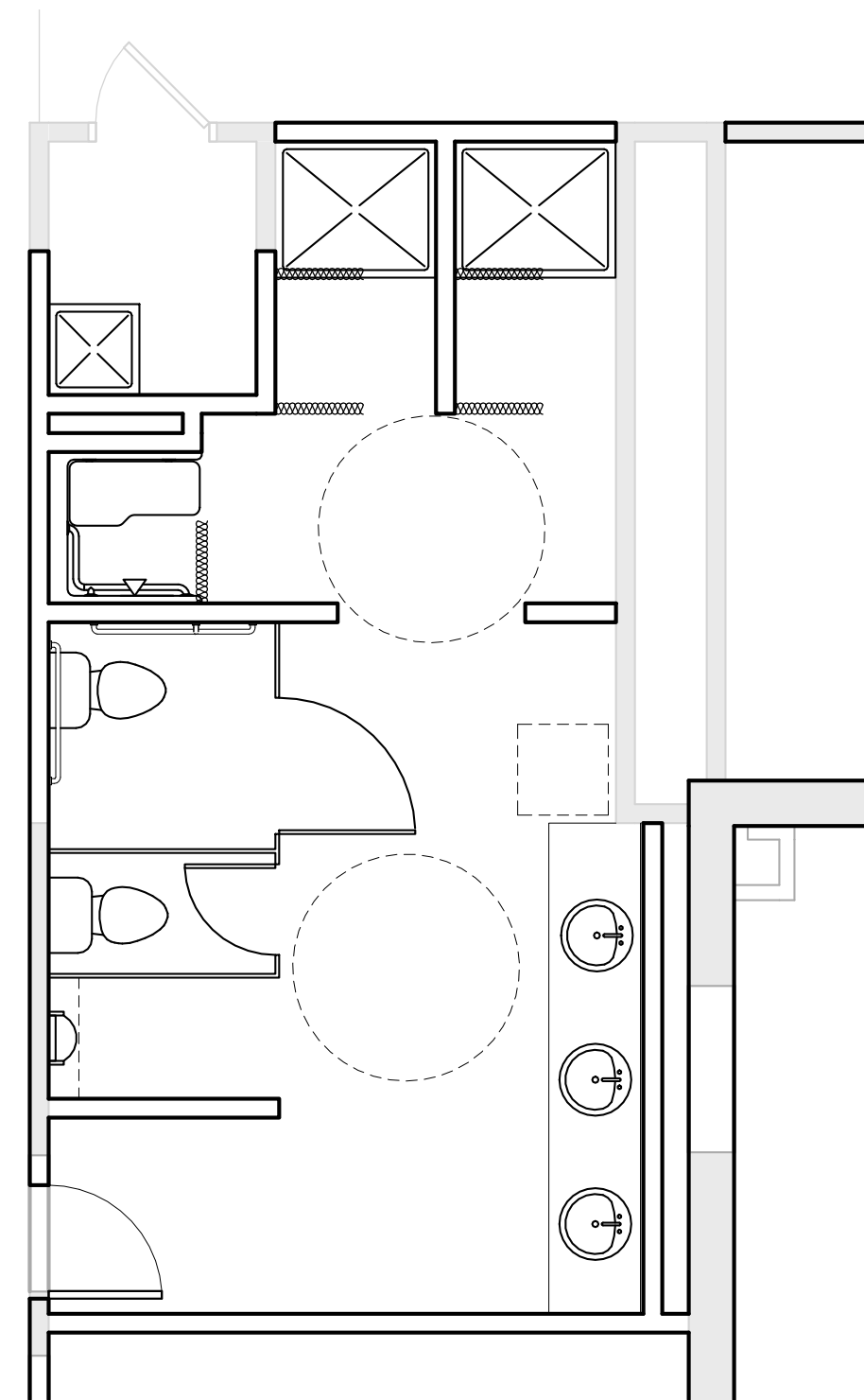
② RESTROOM OPTION 1 1/4" = 1'-0"
